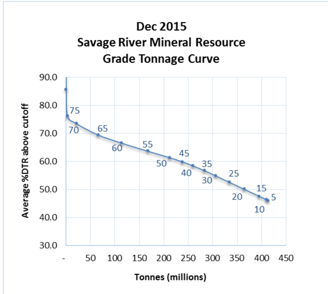
Figure 4 - Grade Tonnage Curve, Savage River
