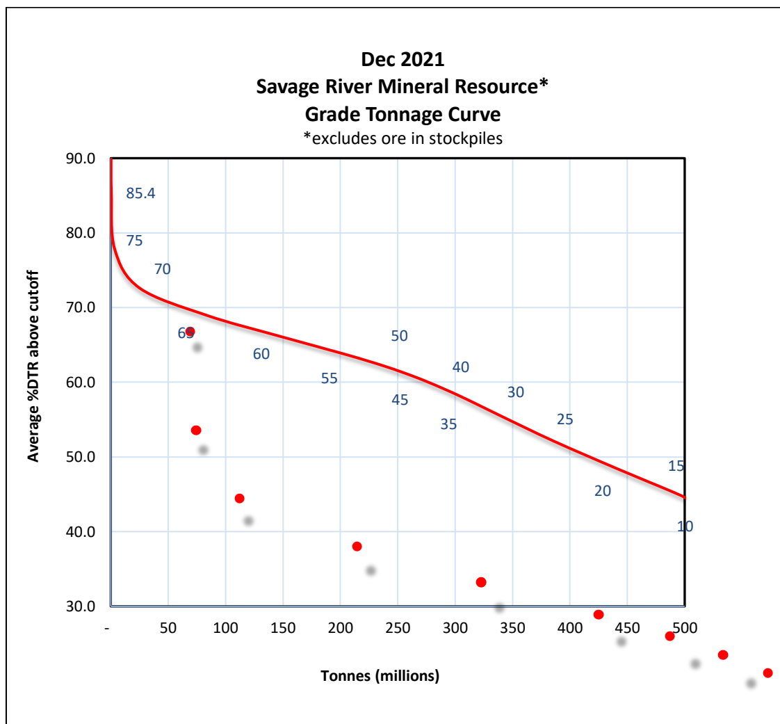
Figure 4 Total Resources Grade Tonnage Curve December 2021
