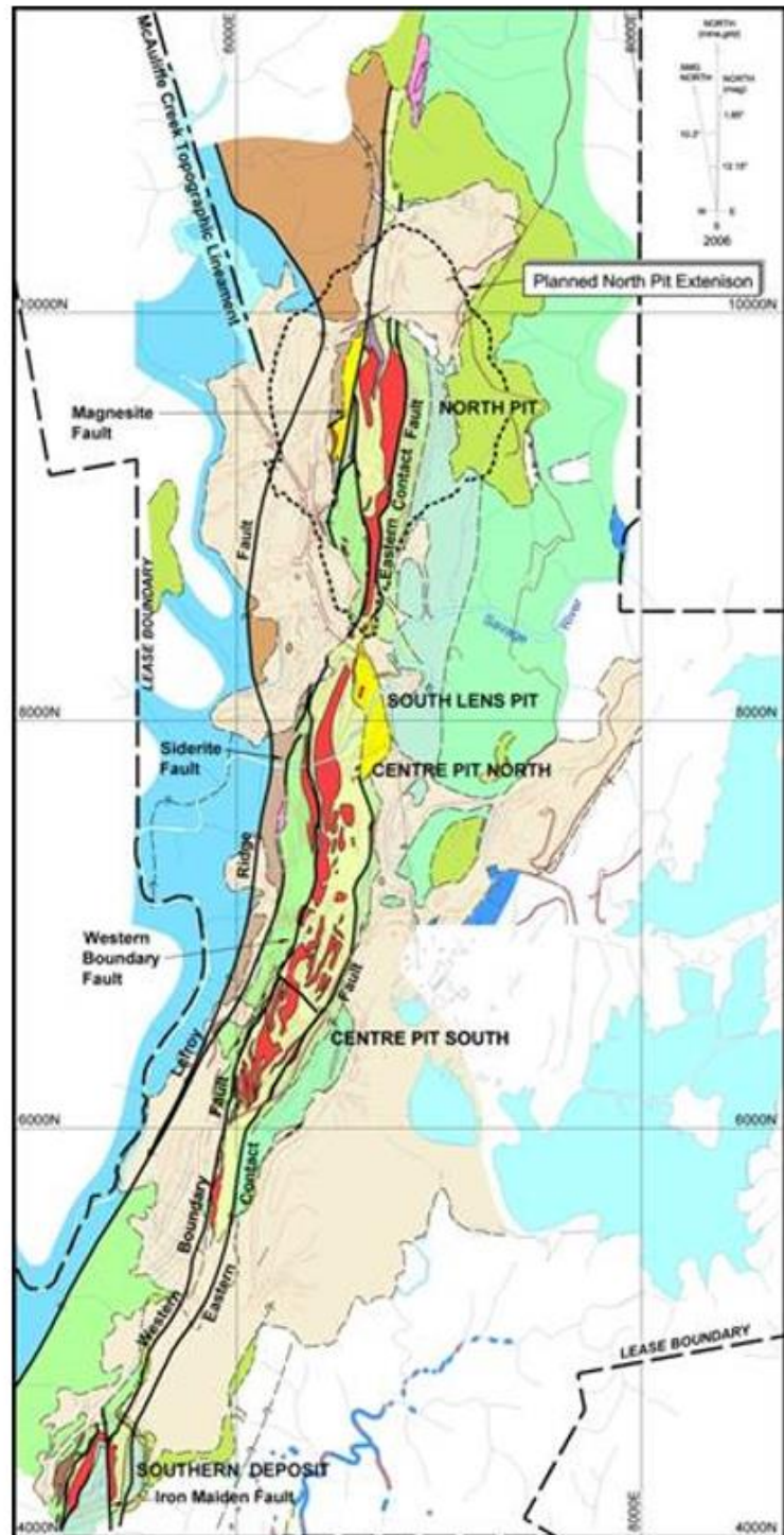
Figure 6 Regional Geology (2008)
